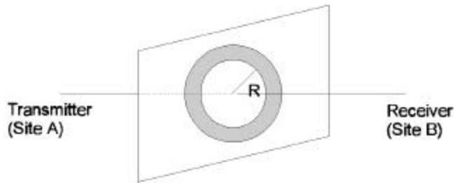
Figure 7: Fresnel Zone
