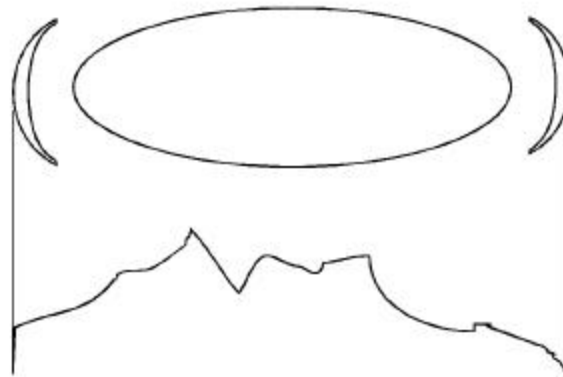
Figure 8: Fresnel Zone Clear of Obstacles
